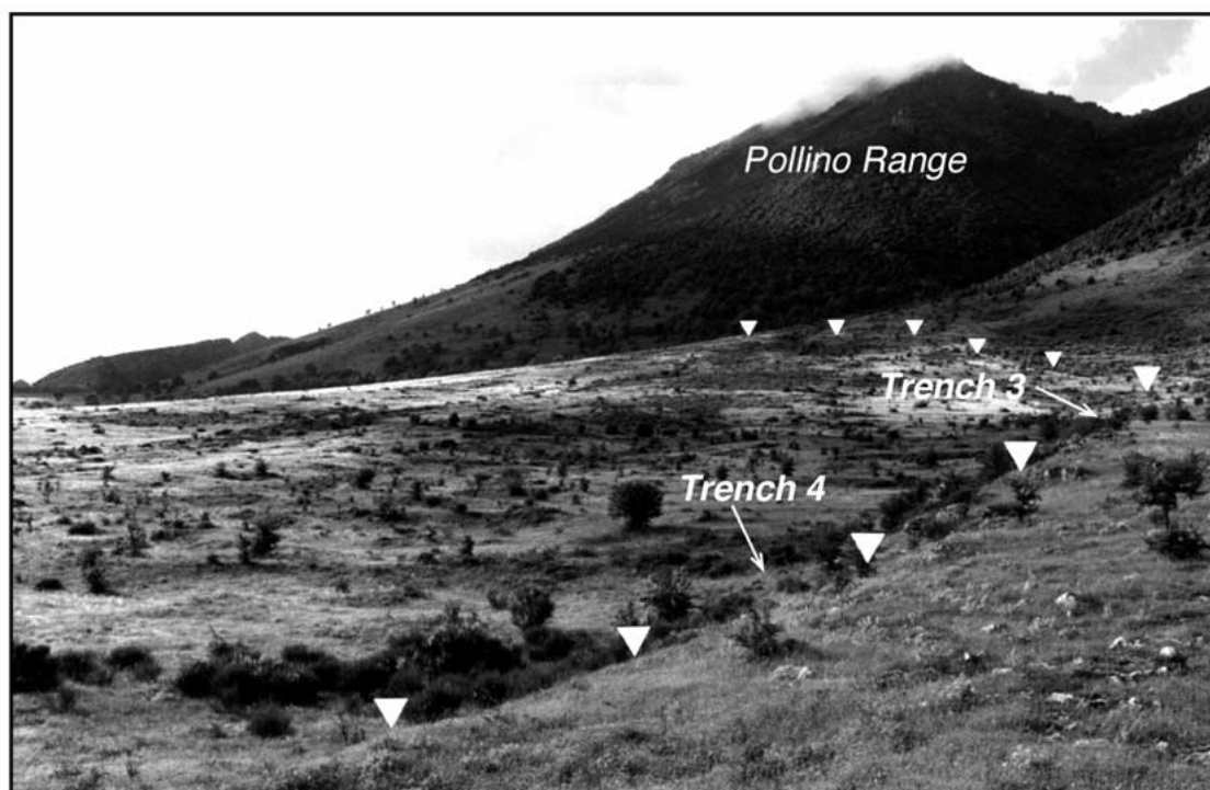
Figure 6. View of the Torre di Giorgio site (see Figure 2 for location). Triangles point to the scarp trace.
