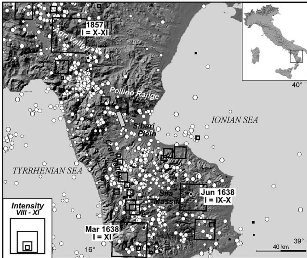
Figure 1. Distribution of historical and instrumental seismicity in southern Italy. White circles represent the instrumental earthquakes ( 2 \leq M \leq 5.3 ) recorded by the Istituto Nazionale di Geofisica between 1984 and 1999. Historical events (Gruppo di Lavoro CPTI, 1999) are indicated by black rectangles; year of occurrence and intensities of the major historical earthquakes are also shown. In the Pollino Range area no large historical event is reported and the instrumental seismicity is rather diffuse. The Castrovillari fault is represented by light grey rectangle.
