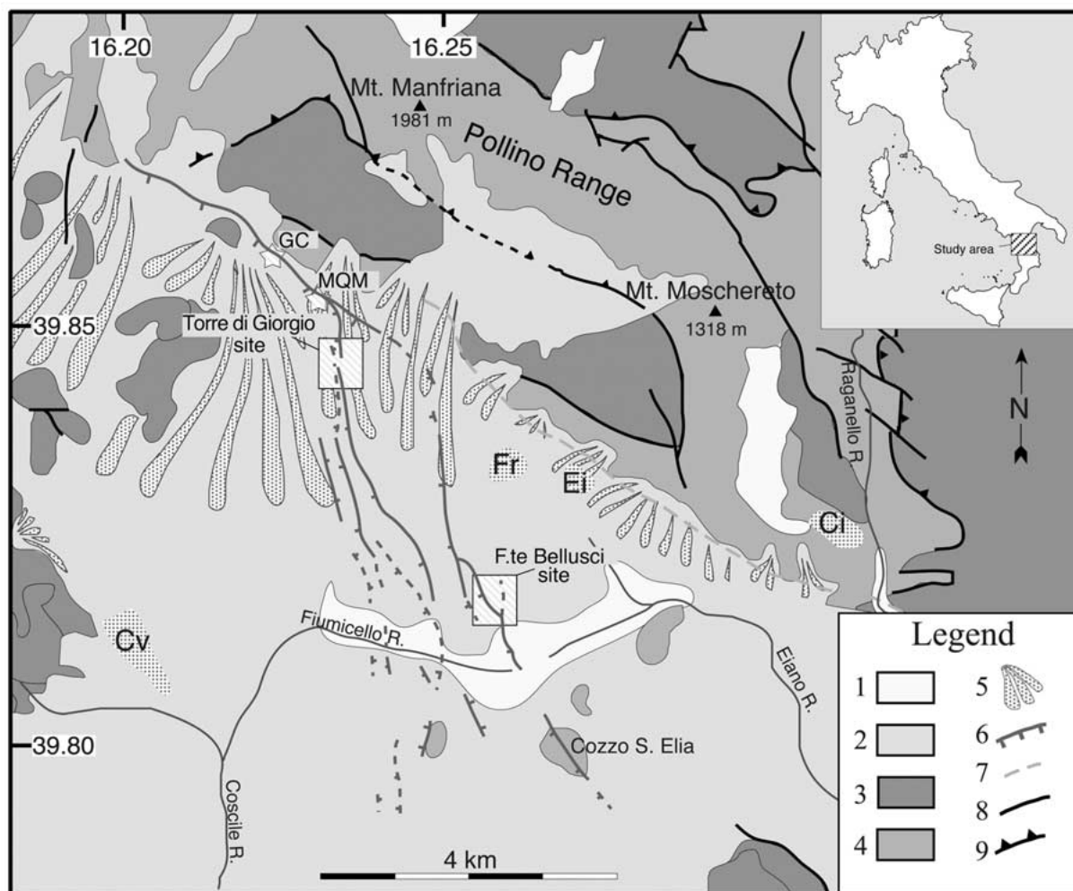
Figure 2. Schematic geological and structural map of the Pollino Range area. The location of the Castrovillari fault scarp system is shown. Boxes indicate the paleoseismological sites from this paper and from Cinti et al., 1997, and stars those from Michetti et al., 1997. Legend: 1. alluvium and slope debris (Holocene); 2. marine sand and clay, gravely-sandy alluvium and conglomerate (fan-delta), continental colluvium and alluvium (Middle-Late Pleistocene); 3. marly-silty clay and sandstone (flysch, Giurassic-Lower Cretaceous); 4. limestone-dolomite-dolomitic limestone (Triassic-Lower Cretaceous); 5. modern and active slope debris and alluvial fan; 6. Castrovillari fault scarp, dashed where inferred; 7. Pollino fault; 8. undetermined fault; 9. thrust, dashed where inferred. Abbreviations: Cv – Castrovillari; Fr – Frascineto; Ei – Eianina; Ci – Civita; MQM – Masseria Quercia Marina; GC – Grotta Carbone.
